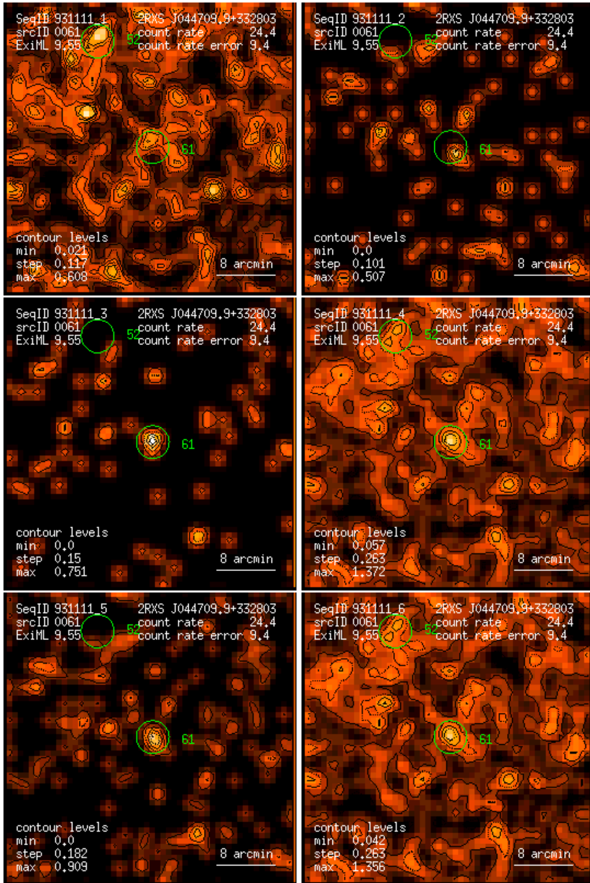
Figure 61: RASS 931111: detection 0061: band rate images, Gaussian filter: (1) PSPC channels 11 – 41, (2) 52 – 90, (3) 91 – 201, (4) 11 – 235, (5) 52 – 201, (6) 11 – 201. Broad band rates in counts/ks. Band rate contour levels in counts/ks/arcmin 2 .
