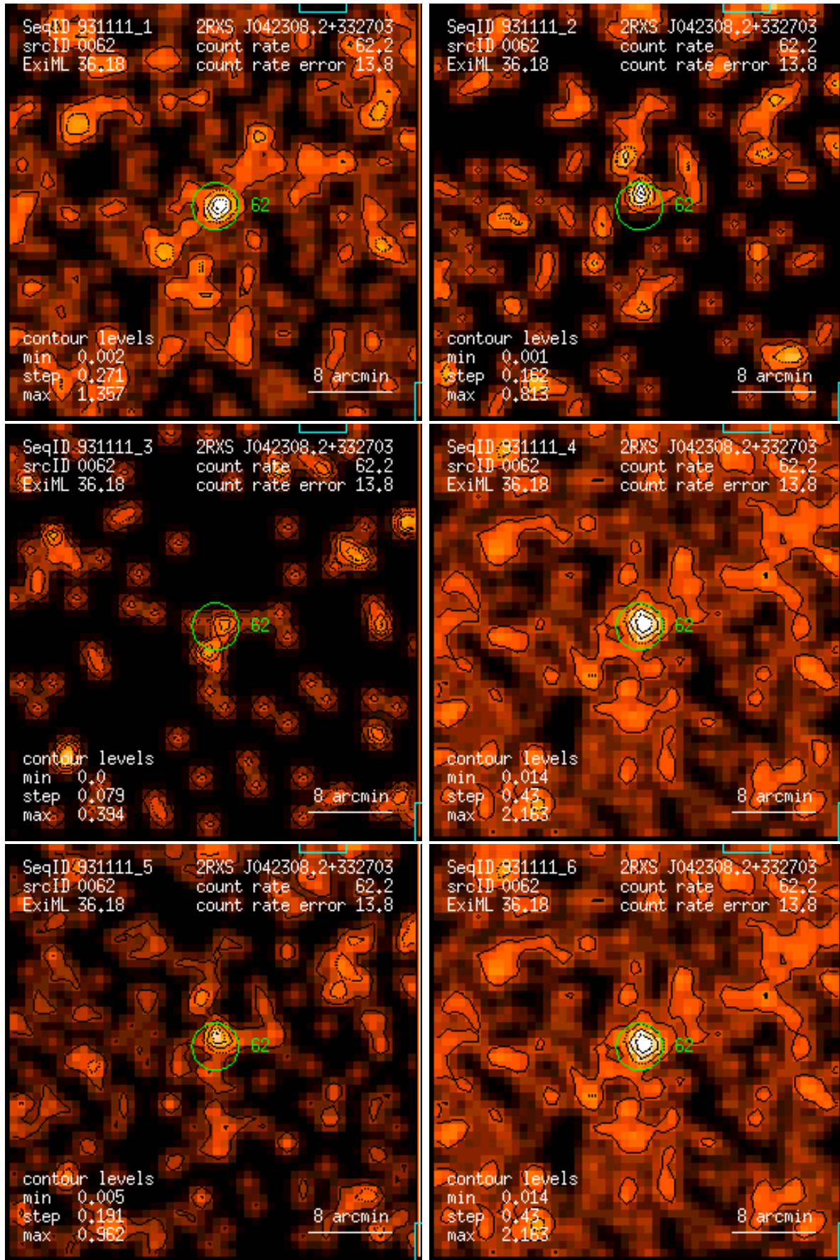
Figure 62: RASS 931111: detection 0062: band rate images, Gaussian filter: (1) PSPC channels 11 – 41, (2) 52 – 90, (3) 91 – 201, (4) 11 – 235, (5) 52 – 201, (6) 11 – 201. Broad band rates in counts/ks. Band rate contour levels in counts/ks/arcmin 2 .
