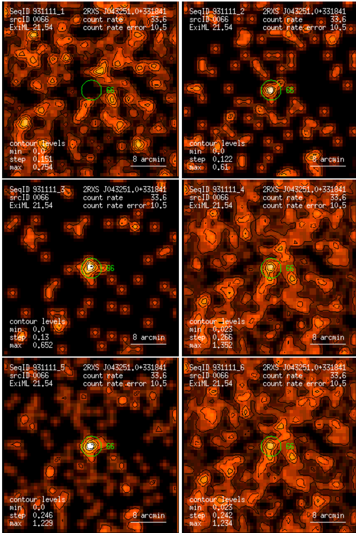
Figure 66: RASS 931111: detection 0066: band rate images, Gaussian filter: (1) PSPC channels 11 – 41, (2) 52 – 90, (3) 91 – 201, (4) 11 – 235, (5) 52 – 201, (6) 11 – 201. Broad band rates in counts/ks. Band rate contour levels in counts/ks/arcmin 2 .
