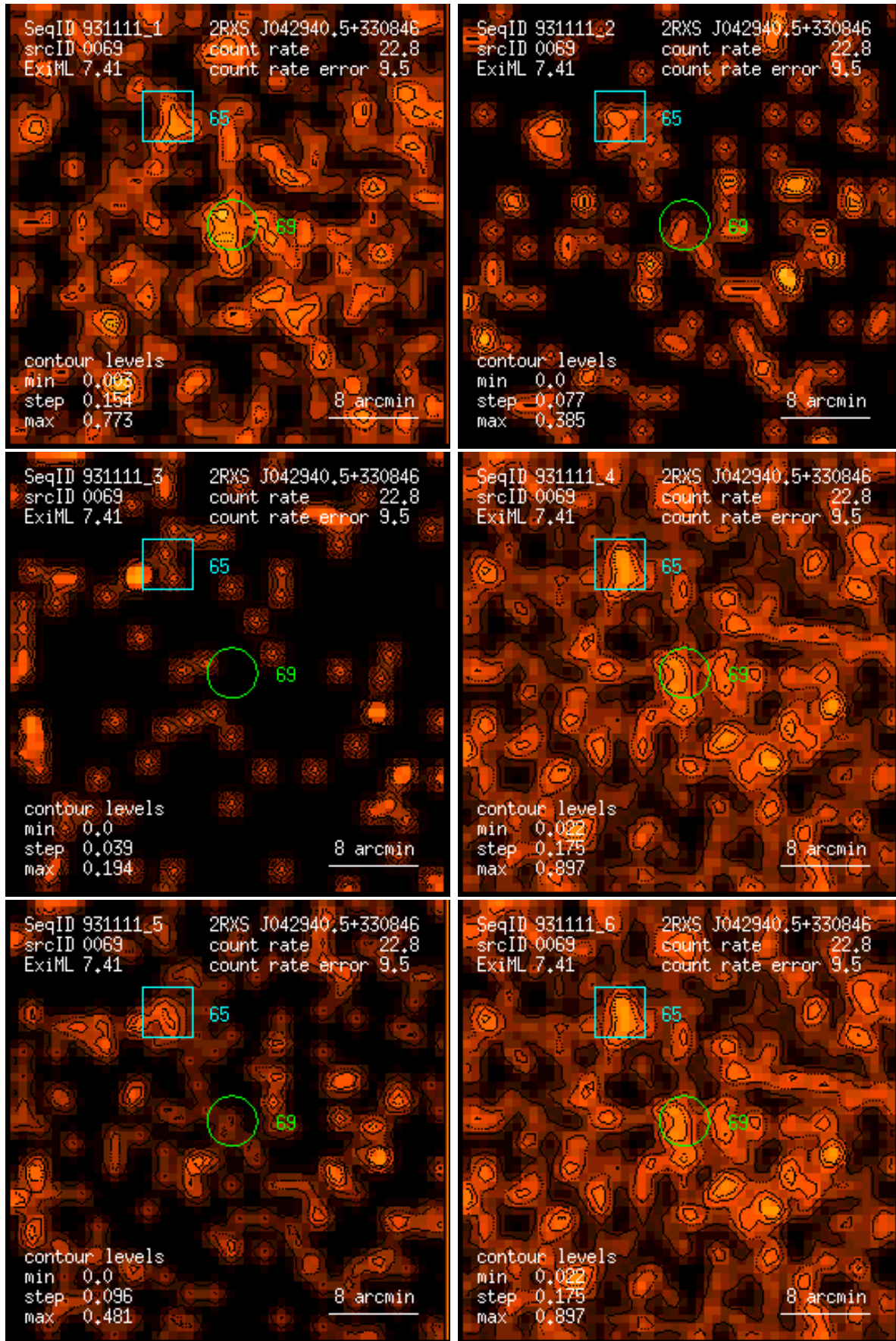
Figure 69: RASS 931111: detection 0069: band rate images, Gaussian filter: (1) PSPC channels 11 – 41, (2) 52 – 90, (3) 91 – 201, (4) 11 – 235, (5) 52 – 201, (6) 11 – 201. Broad band rates in counts/ks. Band rate contour levels in counts/ks/arcmin 2 .
