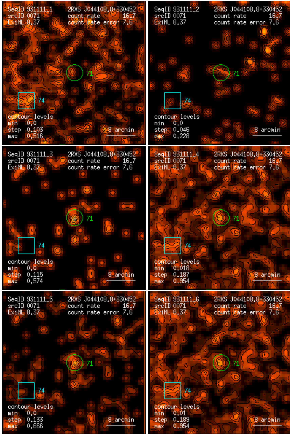
Figure 71: RASS 931111: detection 0071: band rate images, Gaussian filter: (1) PSPC channels 11 – 41, (2) 52 – 90, (3) 91 – 201, (4) 11 – 235, (5) 52 – 201, (6) 11 – 201. Broad band rates in counts/ks. Band rate contour levels in counts/ks/arcmin 2 .
