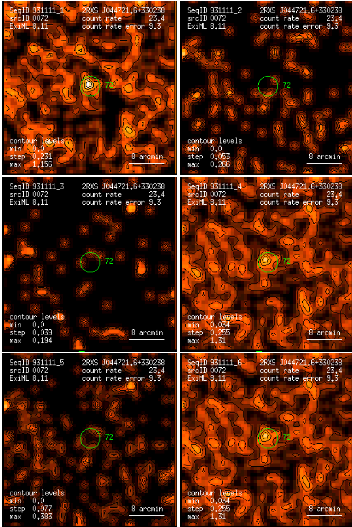
Figure 72: RASS 931111: detection 0072: band rate images, Gaussian filter: (1) PSPC channels 11 – 41, (2) 52 – 90, (3) 91 – 201, (4) 11 – 235, (5) 52 – 201, (6) 11 – 201. Broad band rates in counts/ks. Band rate contour levels in counts/ks/arcmin 2 .
