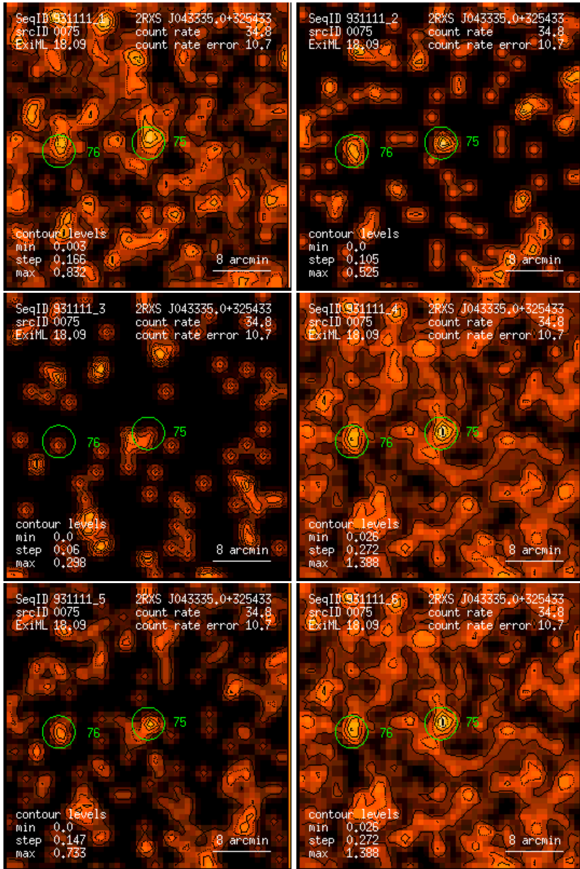
Figure 75: RASS 931111: detection 0075: band rate images, Gaussian filter: (1) PSPC channels 11 – 41, (2) 52 – 90, (3) 91 – 201, (4) 11 – 235, (5) 52 – 201, (6) 11 – 201. Broad band rates in counts/ks. Band rate contour levels in counts/ks/arcmin 2 .
