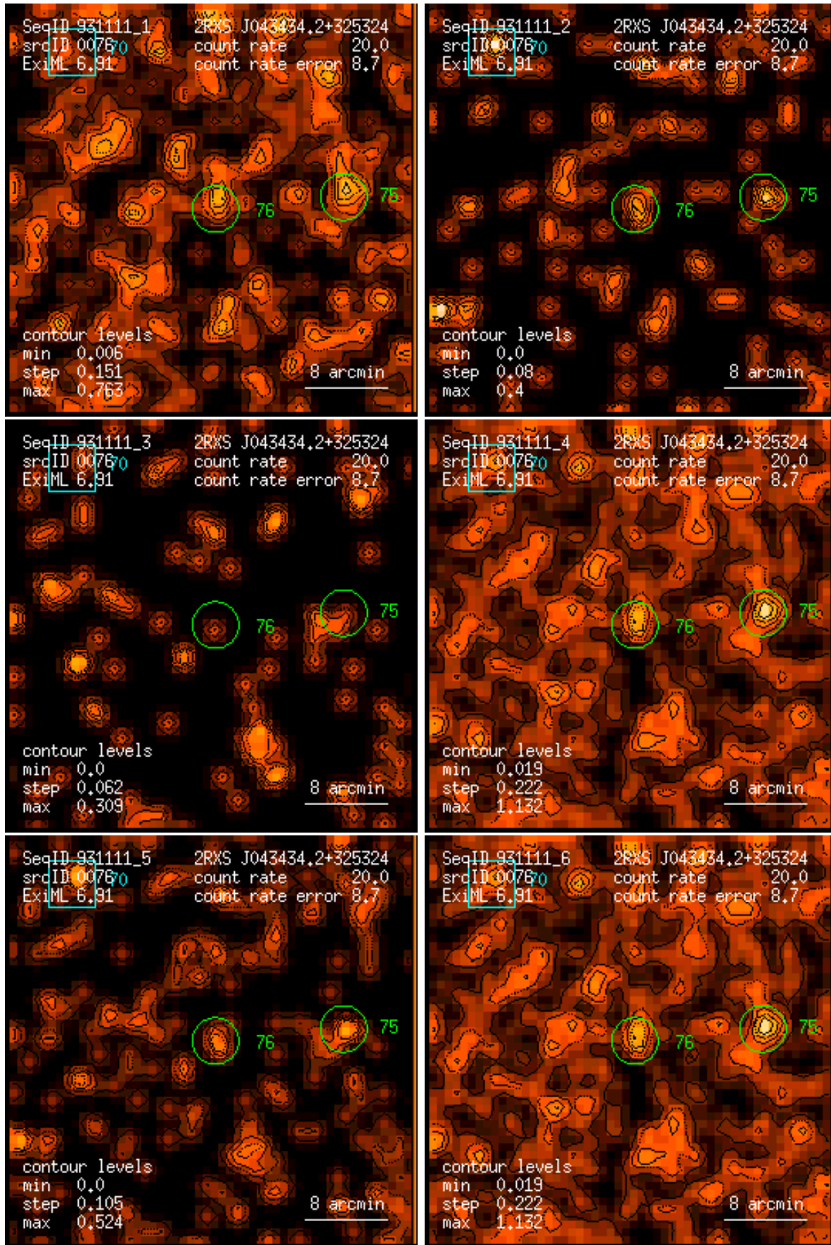
Figure 76: RASS 931111: detection 0076: band rate images, Gaussian filter: (1) PSPC channels 11 – 41, (2) 52 – 90, (3) 91 – 201, (4) 11 – 235, (5) 52 – 201, (6) 11 – 201. Broad band rates in counts/ks. Band rate contour levels in counts/ks/arcmin 2 .
