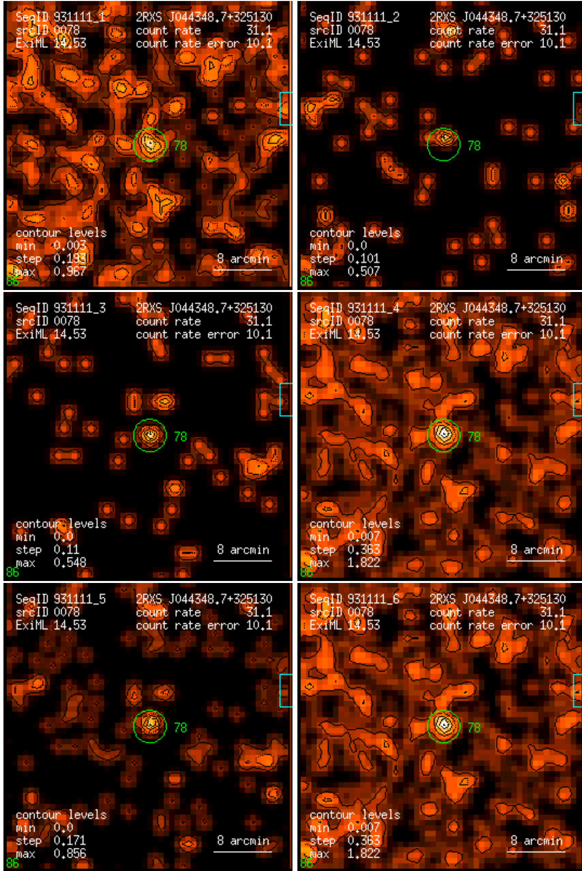
Figure 78: RASS 931111: detection 0078: band rate images, Gaussian filter: (1) PSPC channels 11 – 41, (2) 52 – 90, (3) 91 – 201, (4) 11 – 235, (5) 52 – 201, (6) 11 – 201. Broad band rates in counts/ks. Band rate contour levels in counts/ks/arcmin 2 .
