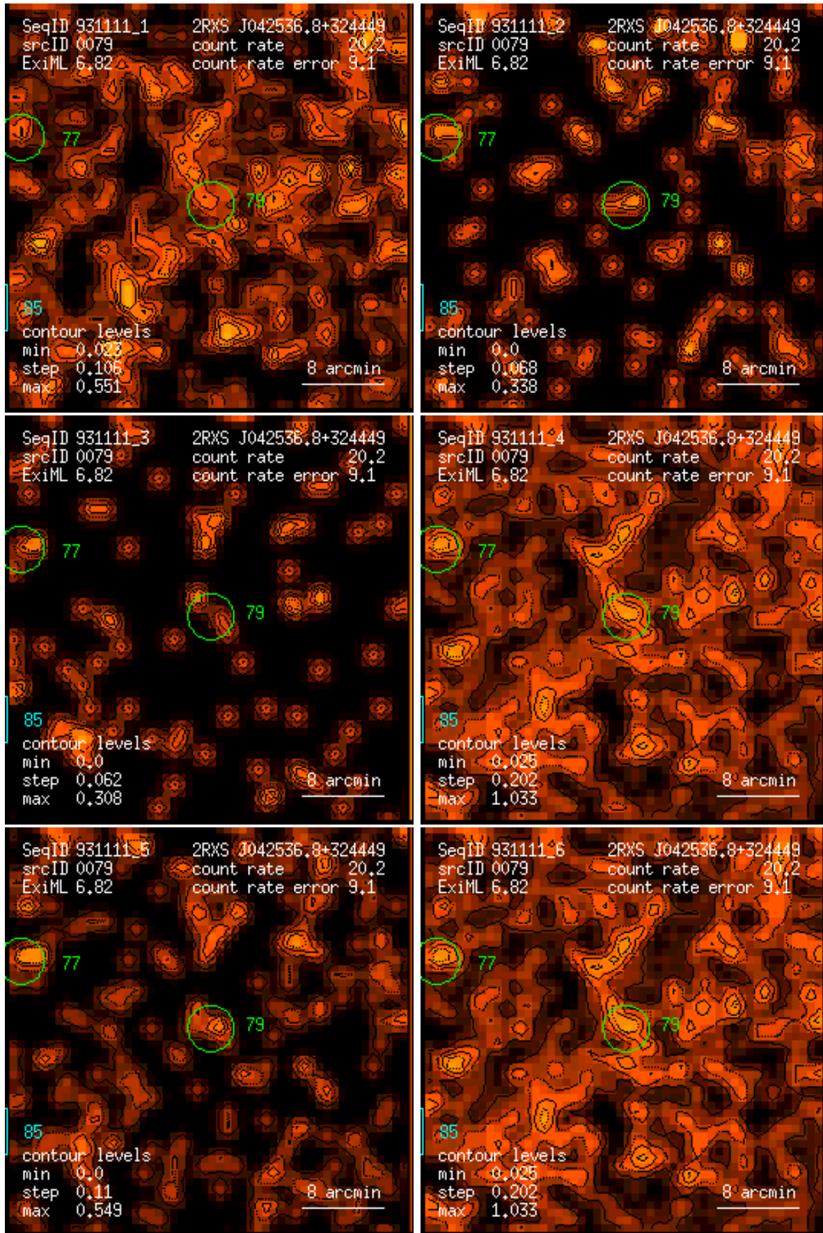
Figure 79: RASS 931111: detection 0079: band rate images, Gaussian filter: (1) PSPC channels 11 – 41, (2) 52 – 90, (3) 91 – 201, (4) 11 – 235, (5) 52 – 201, (6) 11 – 201. Broad band rates in counts/ks. Band rate contour levels in counts/ks/arcmin 2 .
