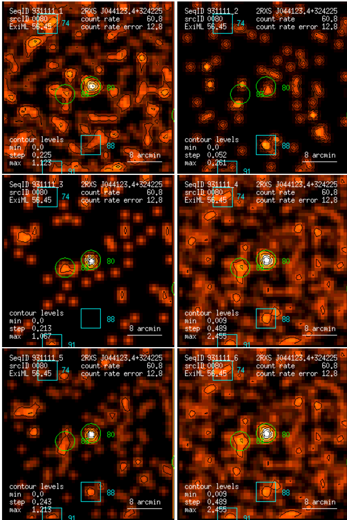
Figure 80: RASS 931111: detection 0080: band rate images, Gaussian filter: (1) PSPC channels 11 – 41, (2) 52 – 90, (3) 91 – 201, (4) 11 – 235, (5) 52 – 201, (6) 11 – 201. Broad band rates in counts/ks. Band rate contour levels in counts/ks/arcmin 2 .
