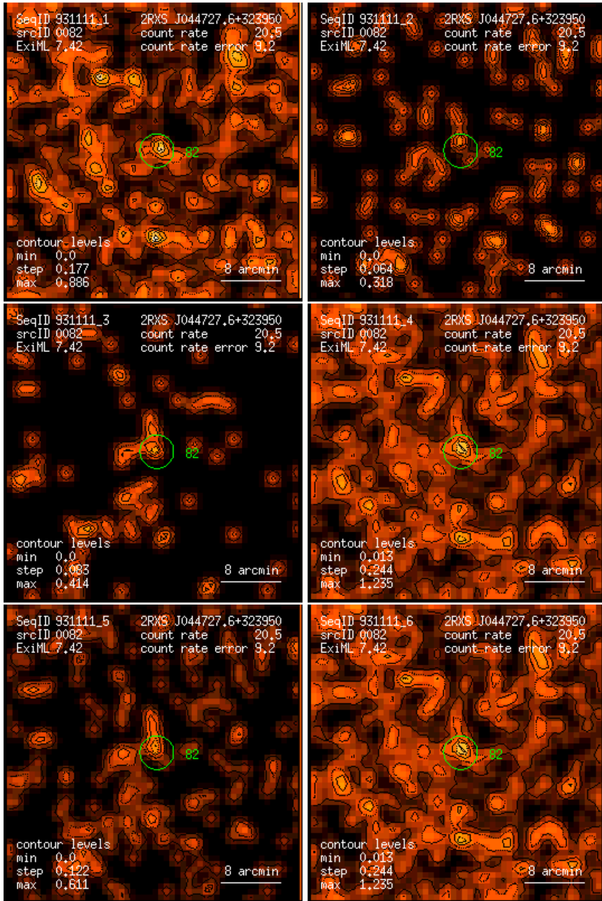
Figure 82: RASS 931111: detection 0082: band rate images, Gaussian filter: (1) PSPC channels 11 – 41, (2) 52 – 90, (3) 91 – 201, (4) 11 – 235, (5) 52 – 201, (6) 11 – 201. Broad band rates in counts/ks. Band rate contour levels in counts/ks/arcmin 2 .
