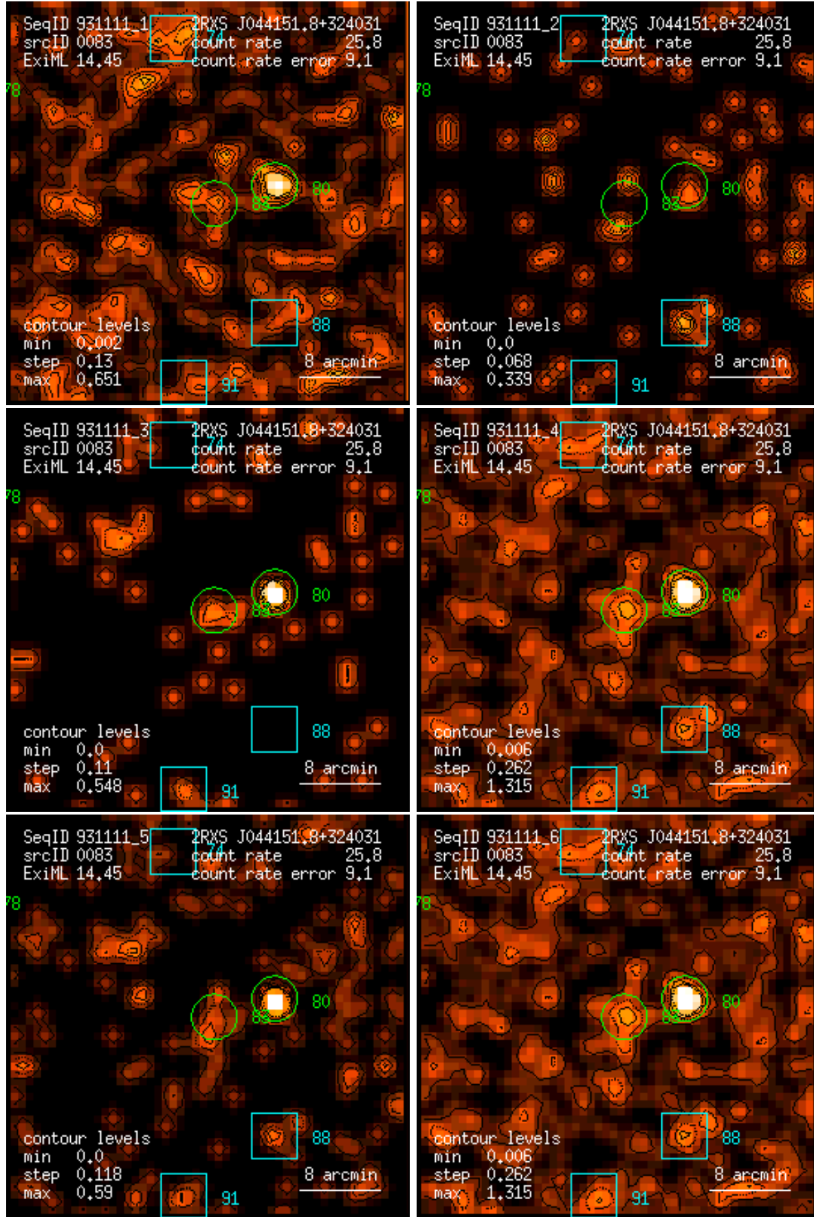
Figure 83: RASS 931111: detection 0083: band rate images, Gaussian filter: (1) PSPC channels 11 – 41, (2) 52 – 90, (3) 91 – 201, (4) 11 – 235, (5) 52 – 201, (6) 11 – 201. Broad band rates in counts/ks. Band rate contour levels in counts/ks/arcmin 2 .
