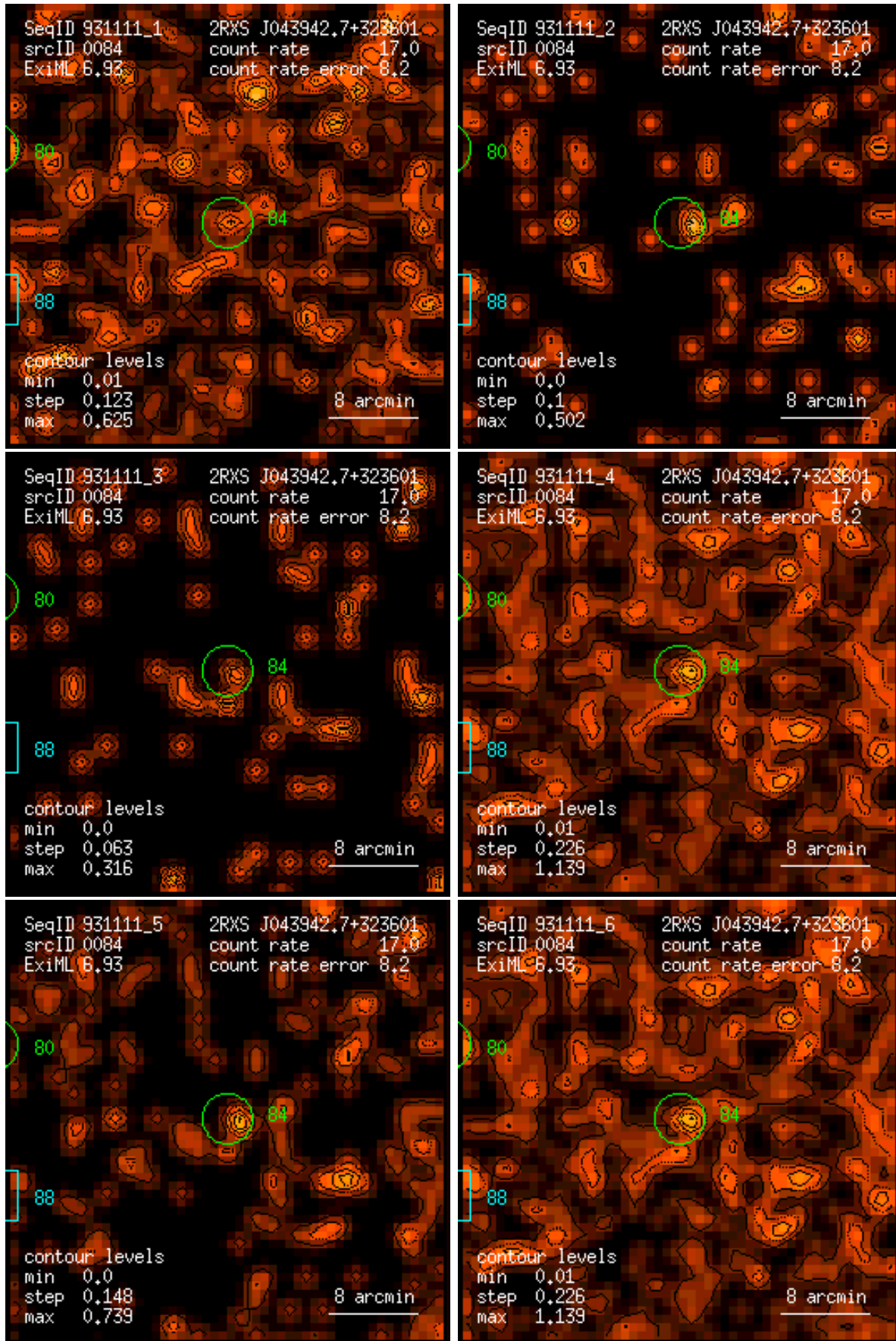
Figure 84: RASS 931111: detection 0084: band rate images, Gaussian filter: (1) PSPC channels 11 – 41, (2) 52 – 90, (3) 91 – 201, (4) 11 – 235, (5) 52 – 201, (6) 11 – 201. Broad band rates in counts/ks. Band rate contour levels in counts/ks/arcmin 2 .
