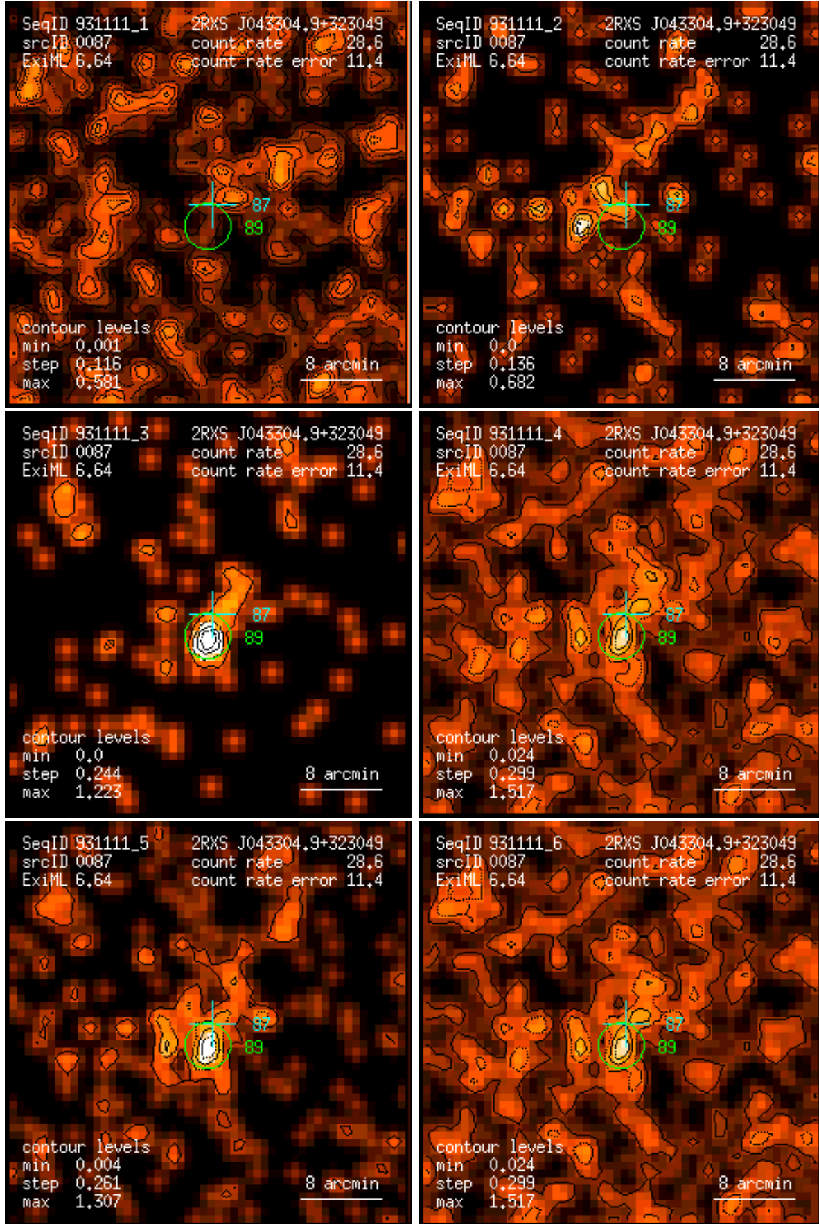
Figure 87: RASS 931111: detection 0087: band rate images, Gaussian filter: (1) PSPC channels 11 – 41, (2) 52 – 90, (3) 91 – 201, (4) 11 – 235, (5) 52 – 201, (6) 11 – 201. Broad band rates in counts/ks. Band rate contour levels in counts/ks/arcmin 2 .
