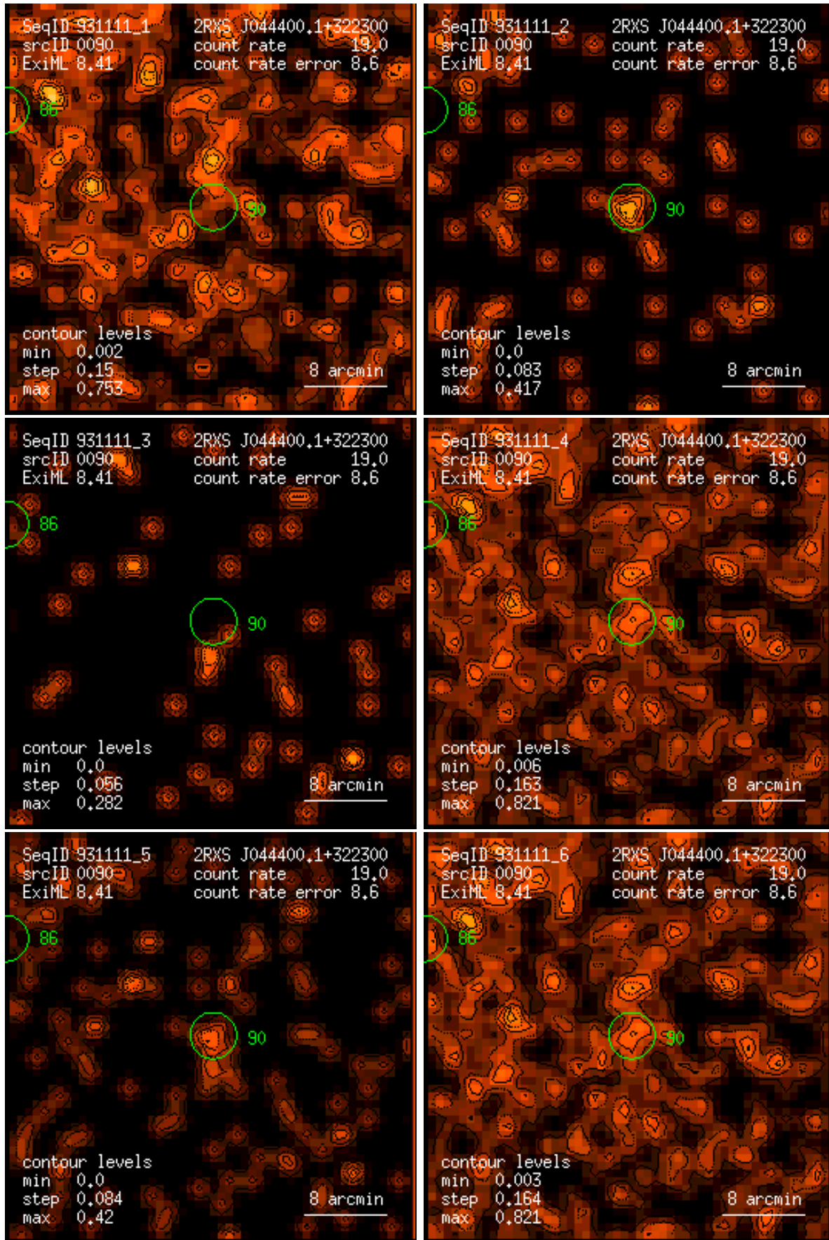
Figure 90: RASS 931111: detection 0090: band rate images, Gaussian filter: (1) PSPC channels 11 – 41, (2) 52 – 90, (3) 91 – 201, (4) 11 – 235, (5) 52 – 201, (6) 11 – 201. Broad band rates in counts/ks. Band rate contour levels in counts/ks/arcmin 2 .
