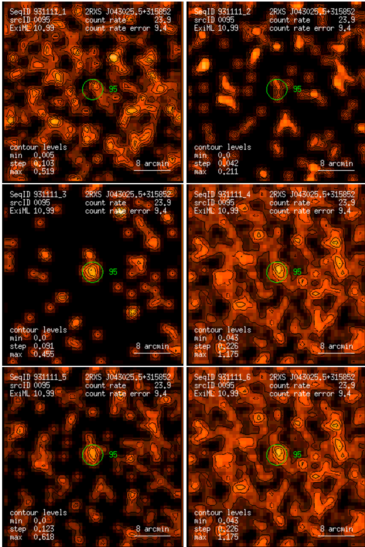
Figure 95: RASS 931111: detection 0095: band rate images, Gaussian filter: (1) PSPC channels 11 – 41, (2) 52 – 90, (3) 91 – 201, (4) 11 – 235, (5) 52 – 201, (6) 11 – 201. Broad band rates in counts/ks. Band rate contour levels in counts/ks/arcmin 2 .
