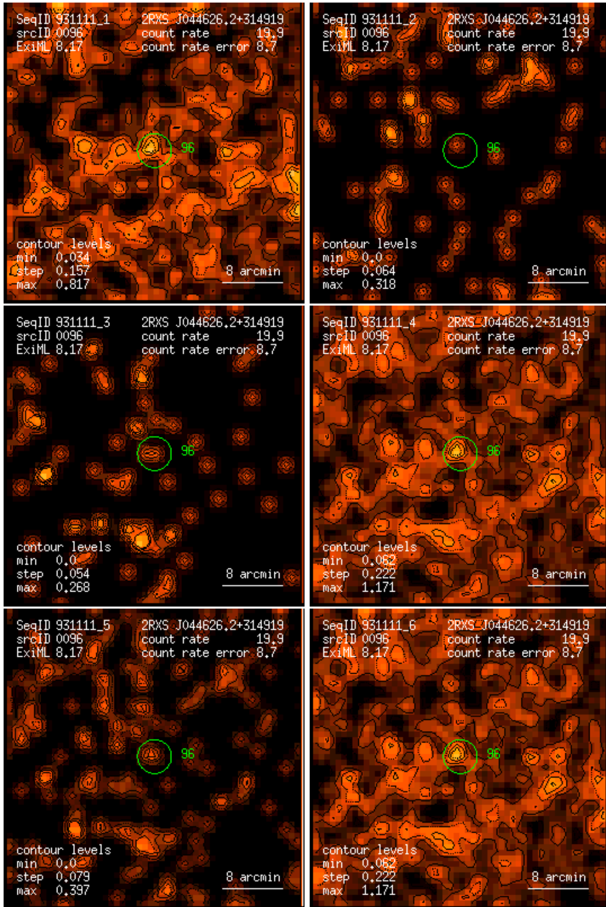
Figure 96: RASS 931111: detection 0096: band rate images, Gaussian filter: (1) PSPC channels 11 – 41, (2) 52 – 90, (3) 91 – 201, (4) 11 – 235, (5) 52 – 201, (6) 11 – 201. Broad band rates in counts/ks. Band rate contour levels in counts/ks/arcmin 2 .
