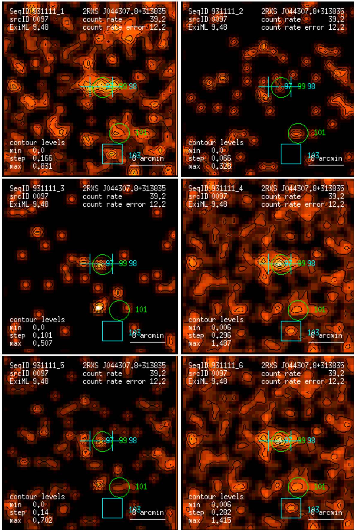
Figure 97: RASS 931111: detection 0097: band rate images, Gaussian filter: (1) PSPC channels 11 – 41, (2) 52 – 90, (3) 91 – 201, (4) 11 – 235, (5) 52 – 201, (6) 11 – 201. Broad band rates in counts/ks. Band rate contour levels in counts/ks/arcmin 2 .
