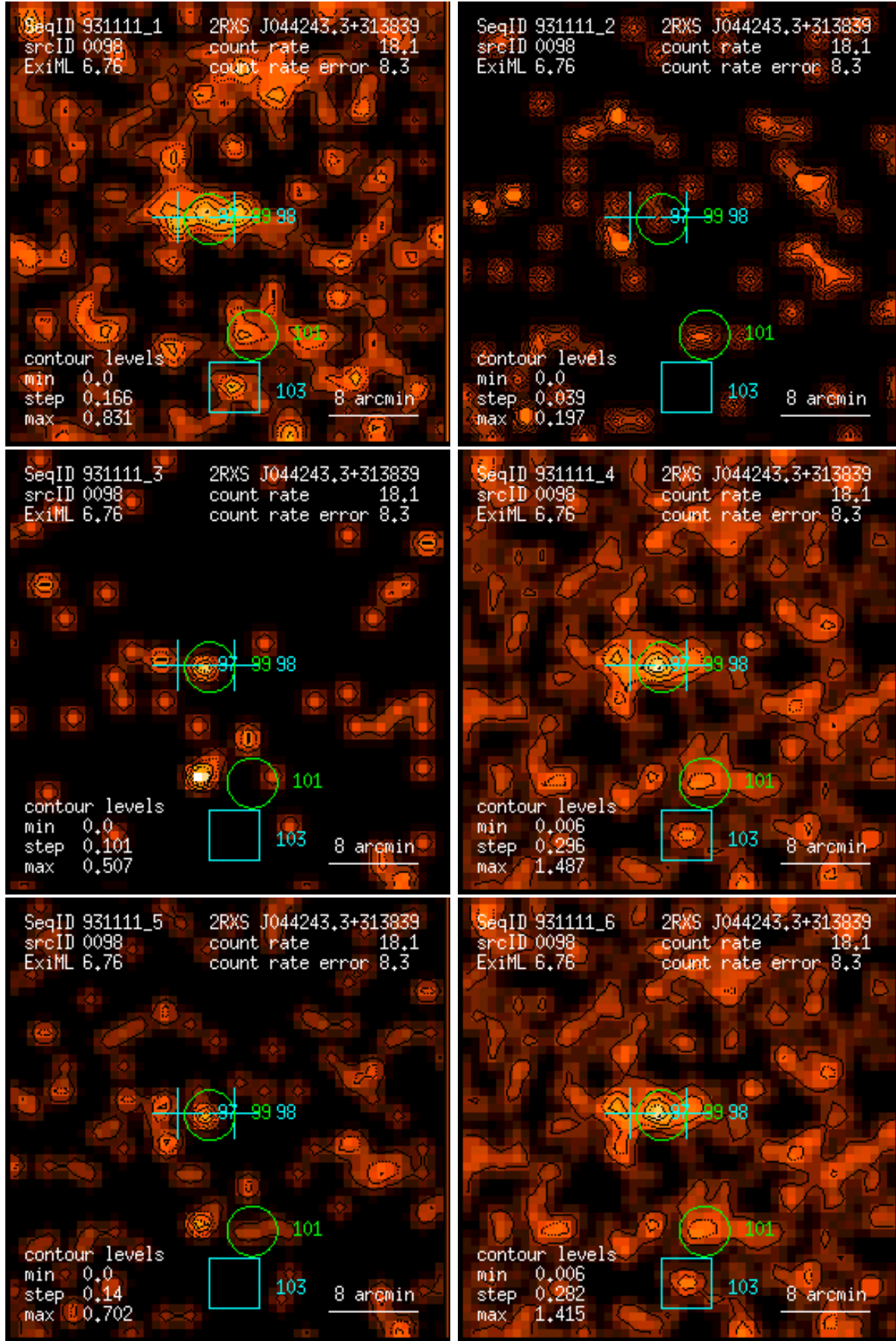
Figure 98: RASS 931111: detection 0098: band rate images, Gaussian filter: (1) PSPC channels 11 – 41, (2) 52 – 90, (3) 91 – 201, (4) 11 – 235, (5) 52 – 201, (6) 11 – 201. Broad band rates in counts/ks. Band rate contour levels in counts/ks/arcmin 2 .
