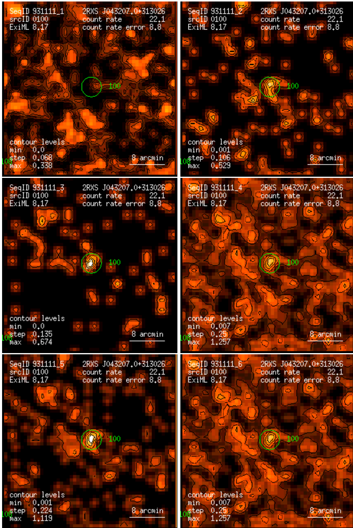
Figure 100: RASS 931111: detection 0100: band rate images, Gaussian filter: (1) PSPC channels 11 – 41, (2) 52 – 90, (3) 91 – 201, (4) 11 – 235, (5) 52 – 201, (6) 11 – 201. Broad band rates in counts/ks. Band rate contour levels in counts/ks/arcmin 2 .
