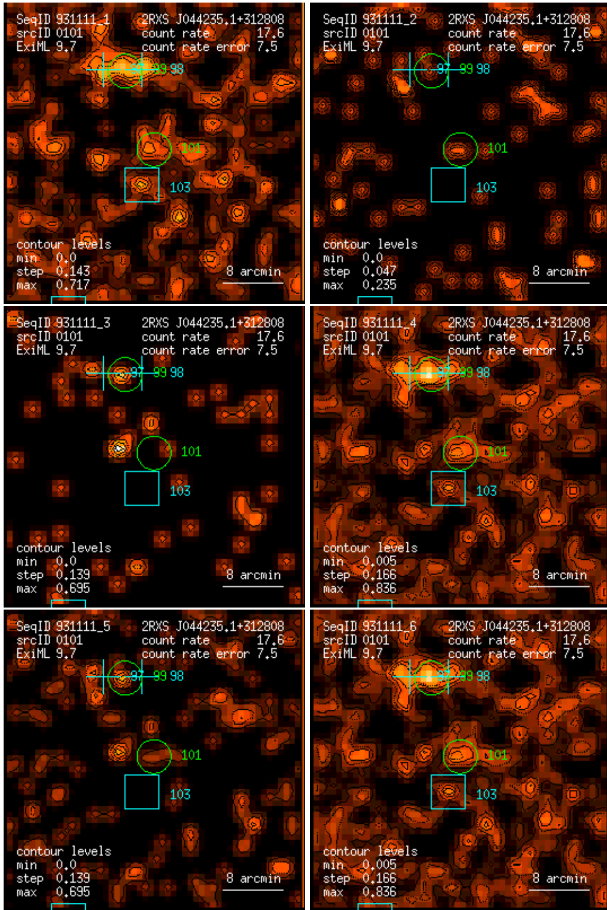
Figure 101: RASS 931111: detection 0101: band rate images, Gaussian filter: (1) PSPC channels 11 – 41, (2) 52 – 90, (3) 91 – 201, (4) 11 – 235, (5) 52 – 201, (6) 11 – 201. Broad band rates in counts/ks. Band rate contour levels in counts/ks/arcmin 2 .
