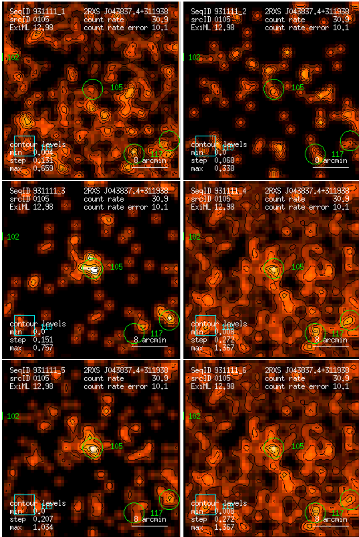
Figure 105: RASS 931111: detection 0105: band rate images, Gaussian filter: (1) PSPC channels 11 – 41, (2) 52 – 90, (3) 91 – 201, (4) 11 – 235, (5) 52 – 201, (6) 11 – 201. Broad band rates in counts/ks. Band rate contour levels in counts/ks/arcmin 2 .
