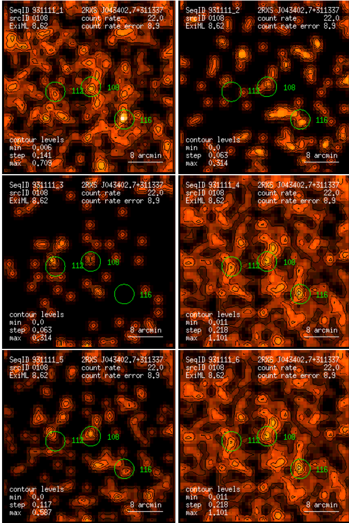
Figure 108: RASS 931111: detection 0108: band rate images, Gaussian filter: (1) PSPC channels 11 – 41, (2) 52 – 90, (3) 91 – 201, (4) 11 – 235, (5) 52 – 201, (6) 11 – 201. Broad band rates in counts/ks. Band rate contour levels in counts/ks/arcmin 2 .
