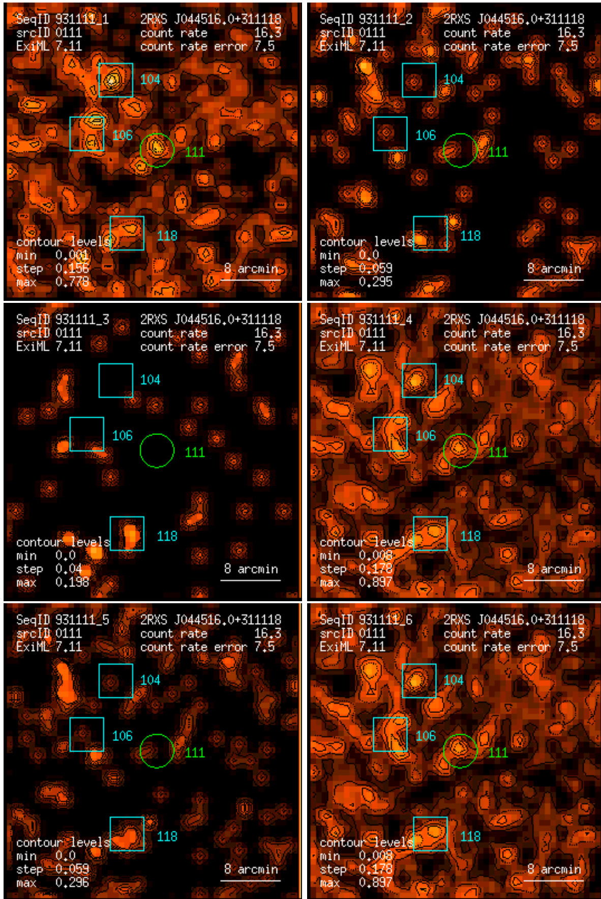
Figure 111: RASS 931111: detection 0111: band rate images, Gaussian filter: (1) PSPC channels 11 – 41, (2) 52 – 90, (3) 91 – 201, (4) 11 – 235, (5) 52 – 201, (6) 11 – 201. Broad band rates in counts/ks. Band rate contour levels in counts/ks/arcmin 2 .
