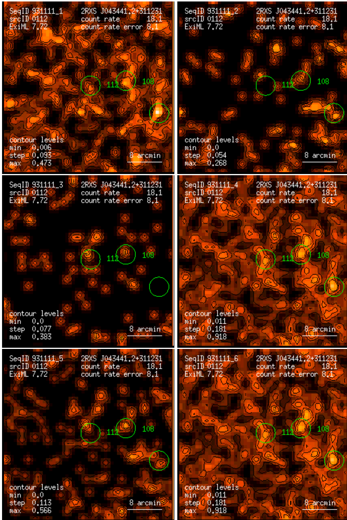
Figure 112: RASS 931111: detection 0112: band rate images, Gaussian filter: (1) PSPC channels 11 – 41, (2) 52 – 90, (3) 91 – 201, (4) 11 – 235, (5) 52 – 201, (6) 11 – 201. Broad band rates in counts/ks. Band rate contour levels in counts/ks/arcmin 2 .
