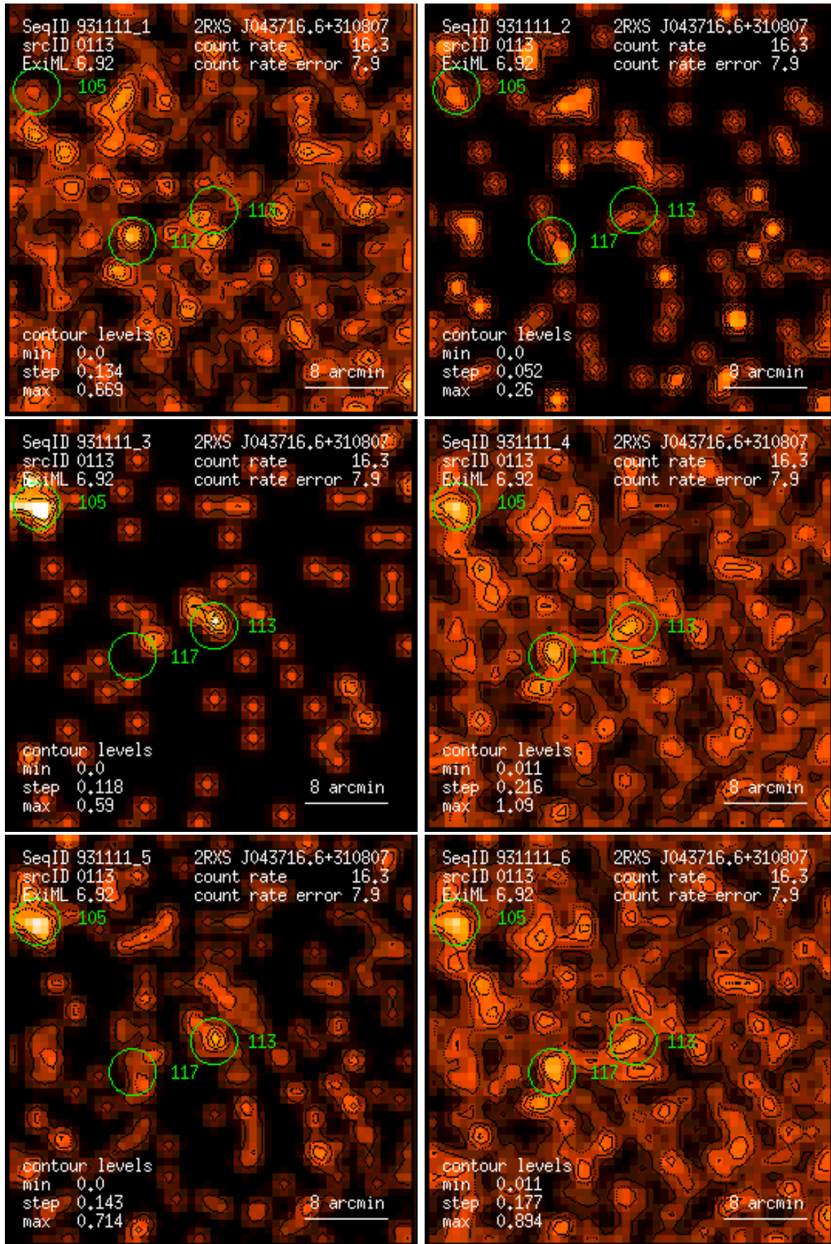
Figure 113: RASS 931111: detection 0113: band rate images, Gaussian filter: (1) PSPC channels 11 – 41, (2) 52 – 90, (3) 91 – 201, (4) 11 – 235, (5) 52 – 201, (6) 11 – 201. Broad band rates in counts/ks. Band rate contour levels in counts/ks/arcmin 2 .
