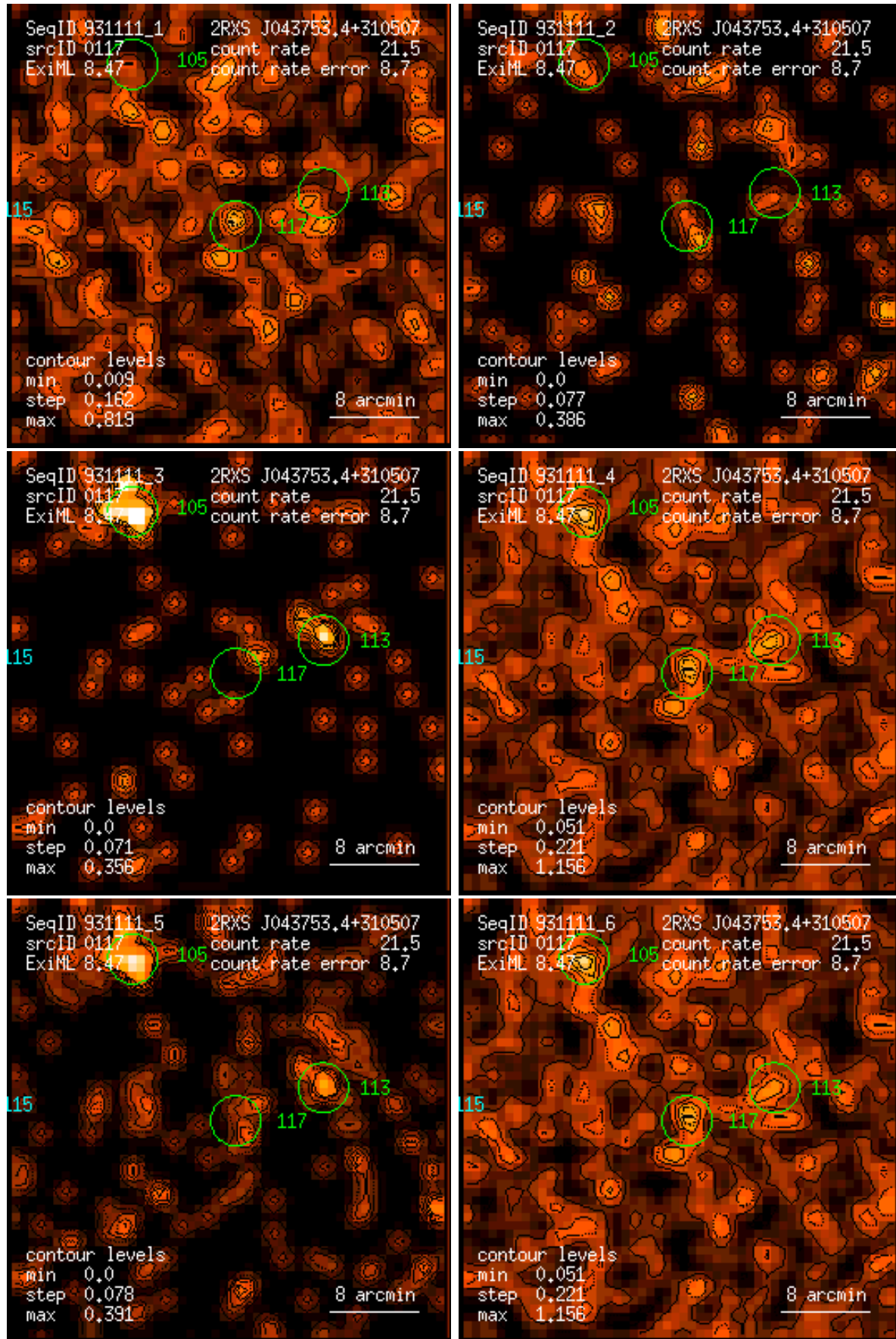
Figure 117: RASS 931111: detection 0117: band rate images, Gaussian filter: (1) PSPC channels 11 – 41, (2) 52 – 90, (3) 91 – 201, (4) 11 – 235, (5) 52 – 201, (6) 11 – 201. Broad band rates in counts/ks. Band rate contour levels in counts/ks/arcmin 2 .
