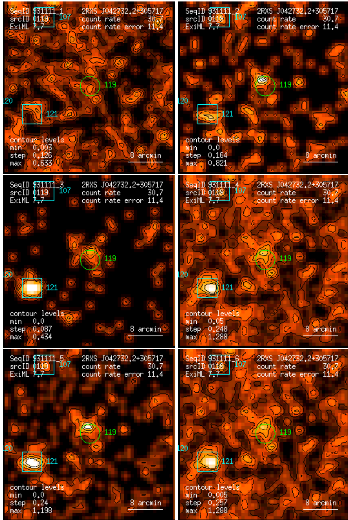
Figure 119: RASS 931111: detection 0119: band rate images, Gaussian filter: (1) PSPC channels 11 – 41, (2) 52 – 90, (3) 91 – 201, (4) 11 – 235, (5) 52 – 201, (6) 11 – 201. Broad band rates in counts/ks. Band rate contour levels in counts/ks/arcmin 2 .
