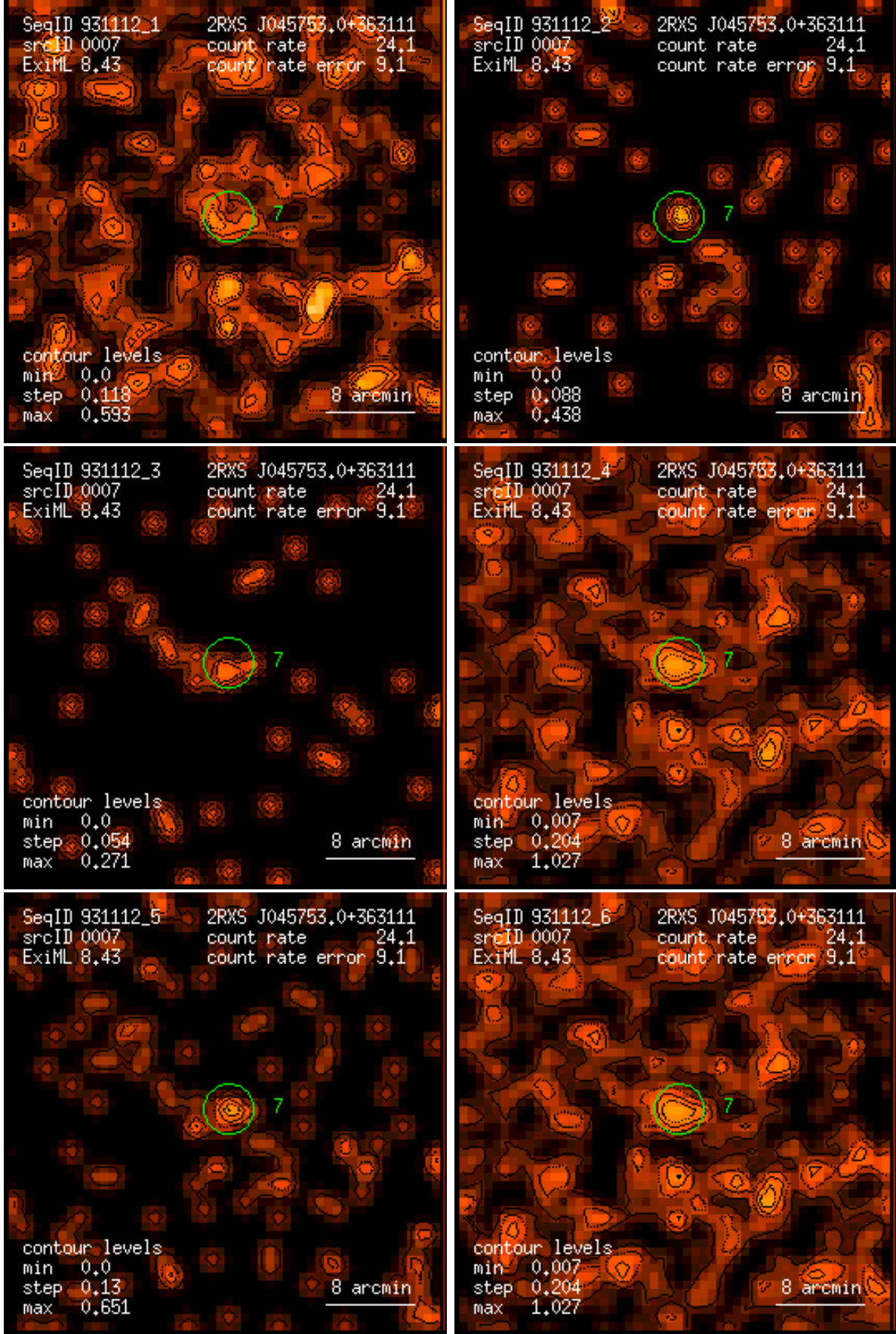
Figure 7: RASS 931112: detection 0007: band rate images, Gaussian filter: (1) PSPC channels 11 – 41, (2) 52 – 90, (3) 91 – 201, (4) 11 – 235, (5) 52 – 201, (6) 11 – 201. Broad band rates in counts/ks. Band rate contour levels in counts/ks/arcmin 2 .
