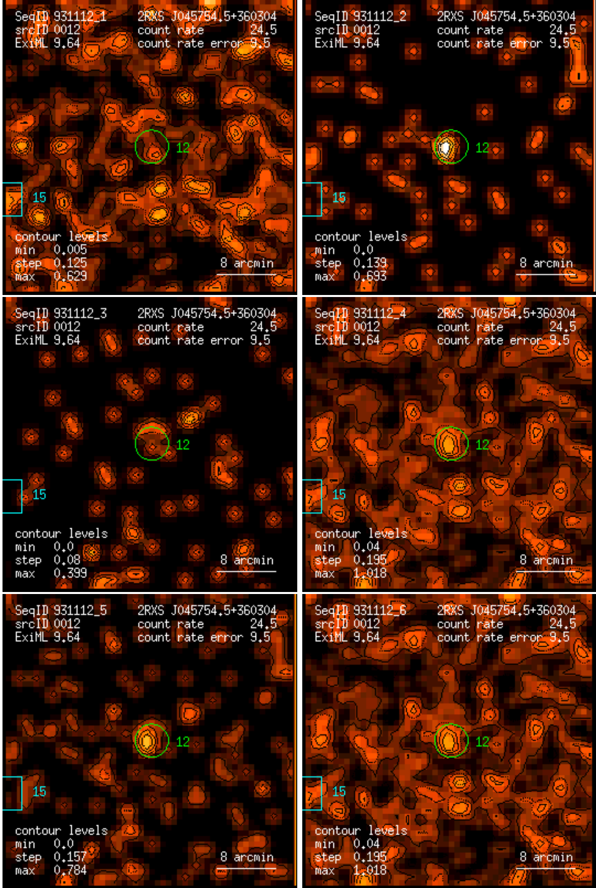
Figure 12: RASS 931112: detection 0012: band rate images, Gaussian filter: (1) PSPC channels 11 – 41, (2) 52 – 90, (3) 91 – 201, (4) 11 – 235, (5) 52 – 201, (6) 11 – 201. Broad band rates in counts/ks. Band rate contour levels in counts/ks/arcmin 2 .
