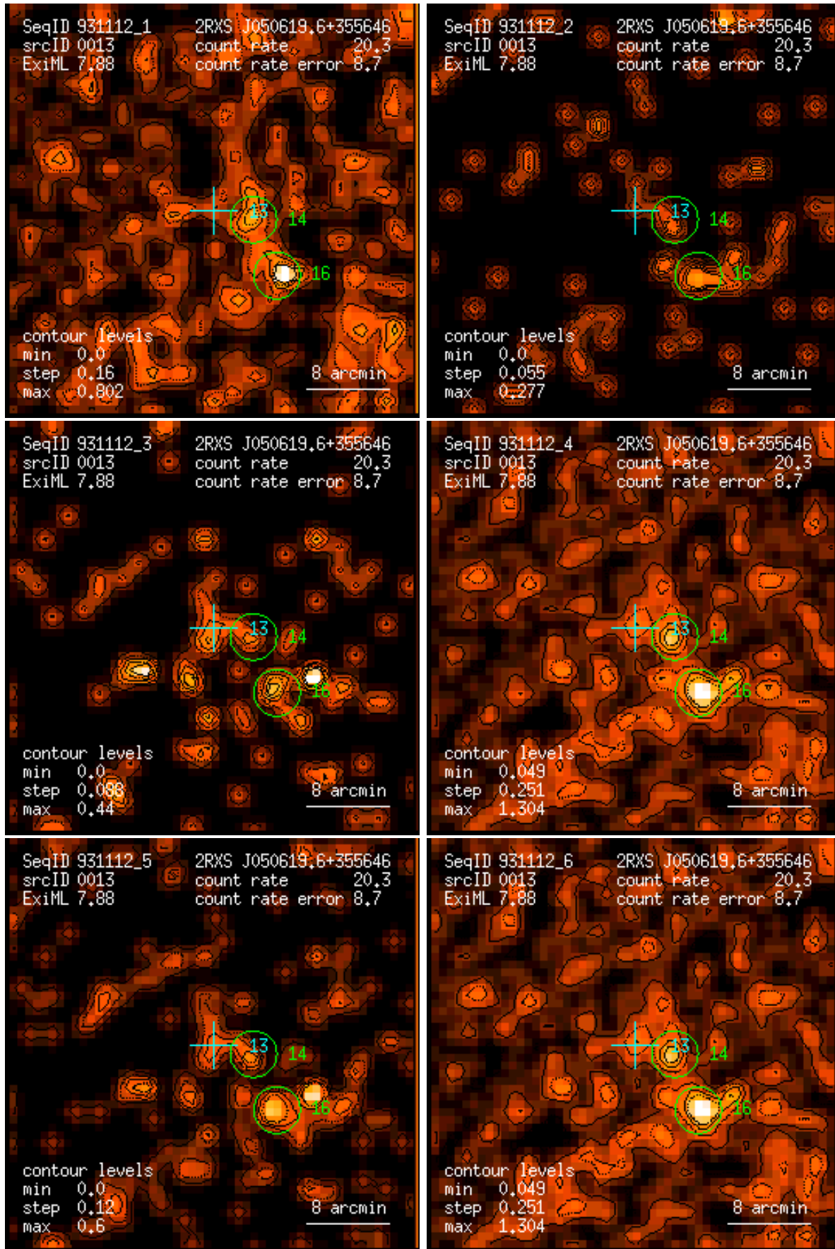
Figure 13: RASS 931112: detection 0013: band rate images, Gaussian filter: (1) PSPC channels 11 – 41, (2) 52 – 90, (3) 91 – 201, (4) 11 – 235, (5) 52 – 201, (6) 11 – 201. Broad band rates in counts/ks. Band rate contour levels in counts/ks/arcmin 2 .
