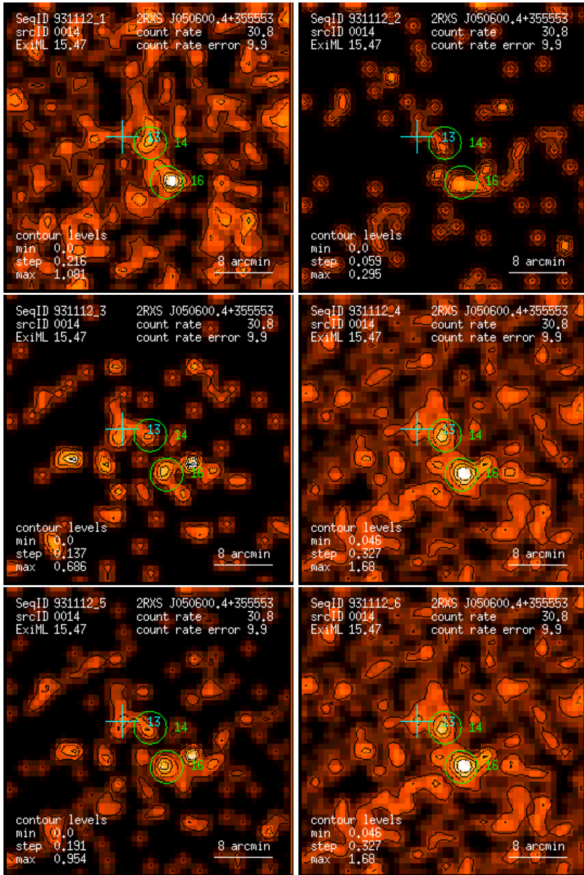
Figure 14: RASS 931112: detection 0014: band rate images, Gaussian filter: (1) PSPC channels 11 – 41, (2) 52 – 90, (3) 91 – 201, (4) 11 – 235, (5) 52 – 201, (6) 11 – 201. Broad band rates in counts/ks. Band rate contour levels in counts/ks/arcmin 2 .
