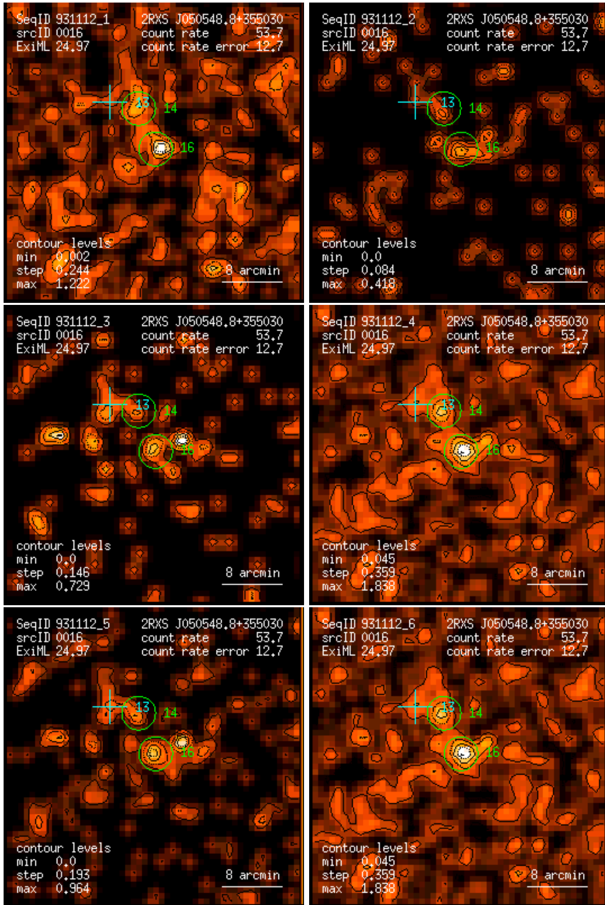
Figure 16: RASS 931112: detection 0016: band rate images, Gaussian filter: (1) PSPC channels 11 – 41, (2) 52 – 90, (3) 91 – 201, (4) 11 – 235, (5) 52 – 201, (6) 11 – 201. Broad band rates in counts/ks. Band rate contour levels in counts/ks/arcmin 2 .
