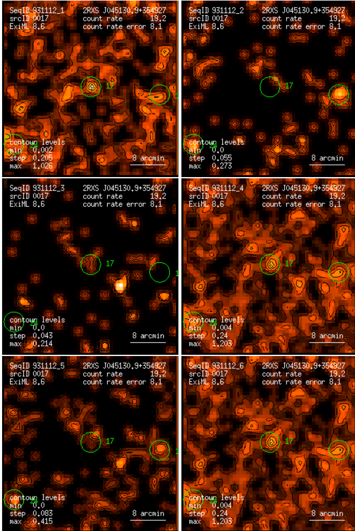
Figure 17: RASS 931112: detection 0017: band rate images, Gaussian filter: (1) PSPC channels 11 – 41, (2) 52 – 90, (3) 91 – 201, (4) 11 – 235, (5) 52 – 201, (6) 11 – 201. Broad band rates in counts/ks. Band rate contour levels in counts/ks/arcmin 2 .
