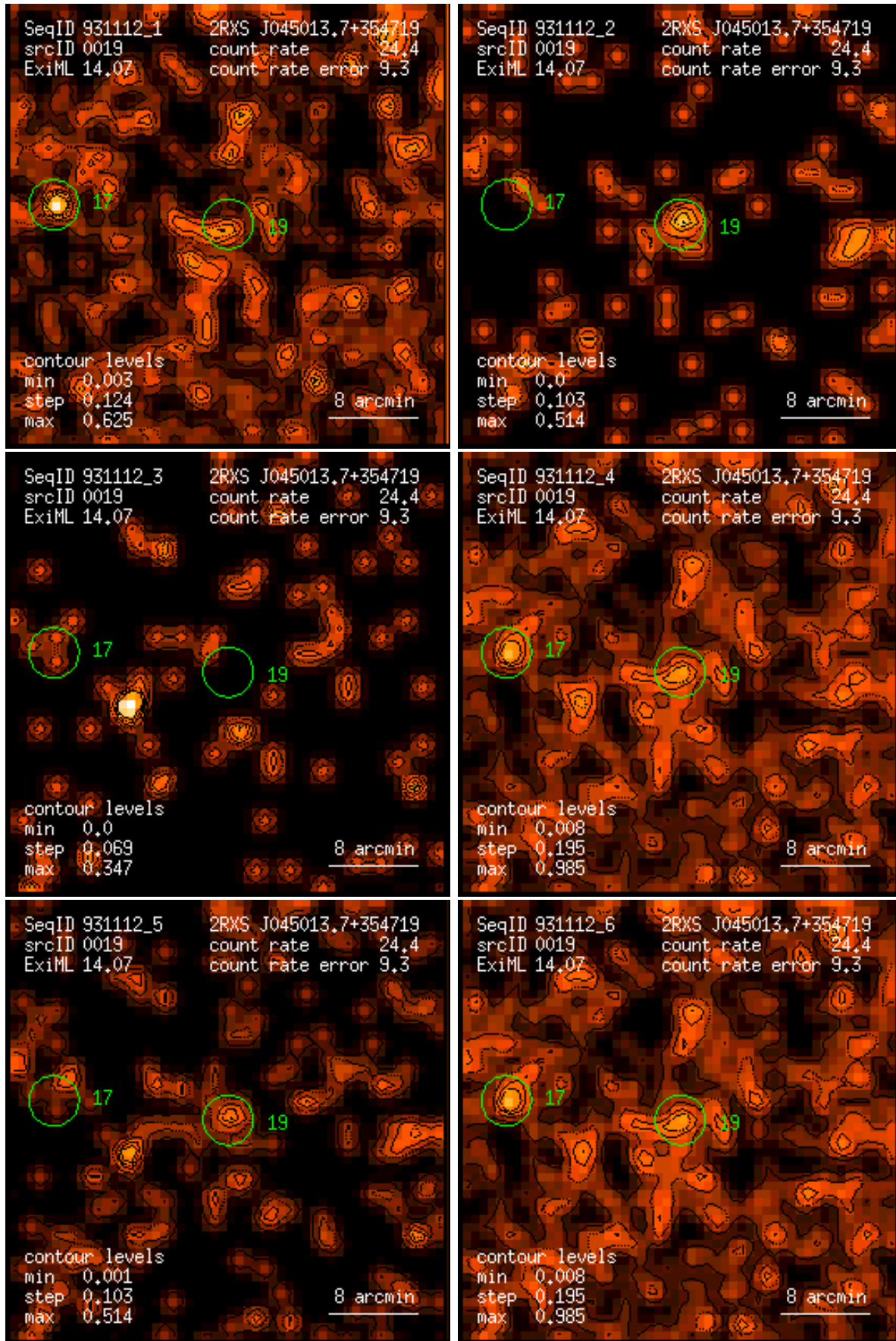
Figure 19: RASS 931112: detection 0019: band rate images, Gaussian filter: (1) PSPC channels 11 – 41, (2) 52 – 90, (3) 91 – 201, (4) 11 – 235, (5) 52 – 201, (6) 11 – 201. Broad band rates in counts/ks. Band rate contour levels in counts/ks/arcmin 2 .
