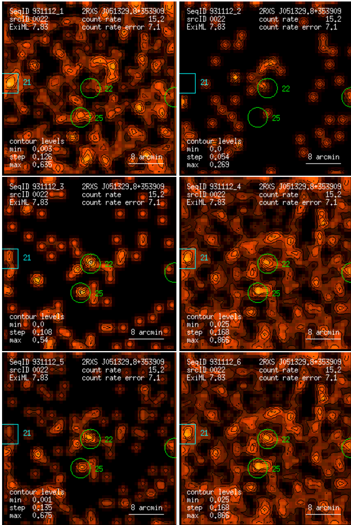
Figure 22: RASS 931112: detection 0022: band rate images, Gaussian filter: (1) PSPC channels 11 – 41, (2) 52 – 90, (3) 91 – 201, (4) 11 – 235, (5) 52 – 201, (6) 11 – 201. Broad band rates in counts/ks. Band rate contour levels in counts/ks/arcmin 2 .
