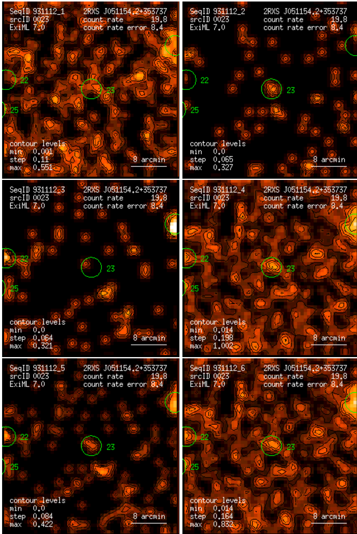
Figure 23: RASS 931112: detection 0023: band rate images, Gaussian filter: (1) PSPC channels 11 – 41, (2) 52 – 90, (3) 91 – 201, (4) 11 – 235, (5) 52 – 201, (6) 11 – 201. Broad band rates in counts/ks. Band rate contour levels in counts/ks/arcmin 2 .
