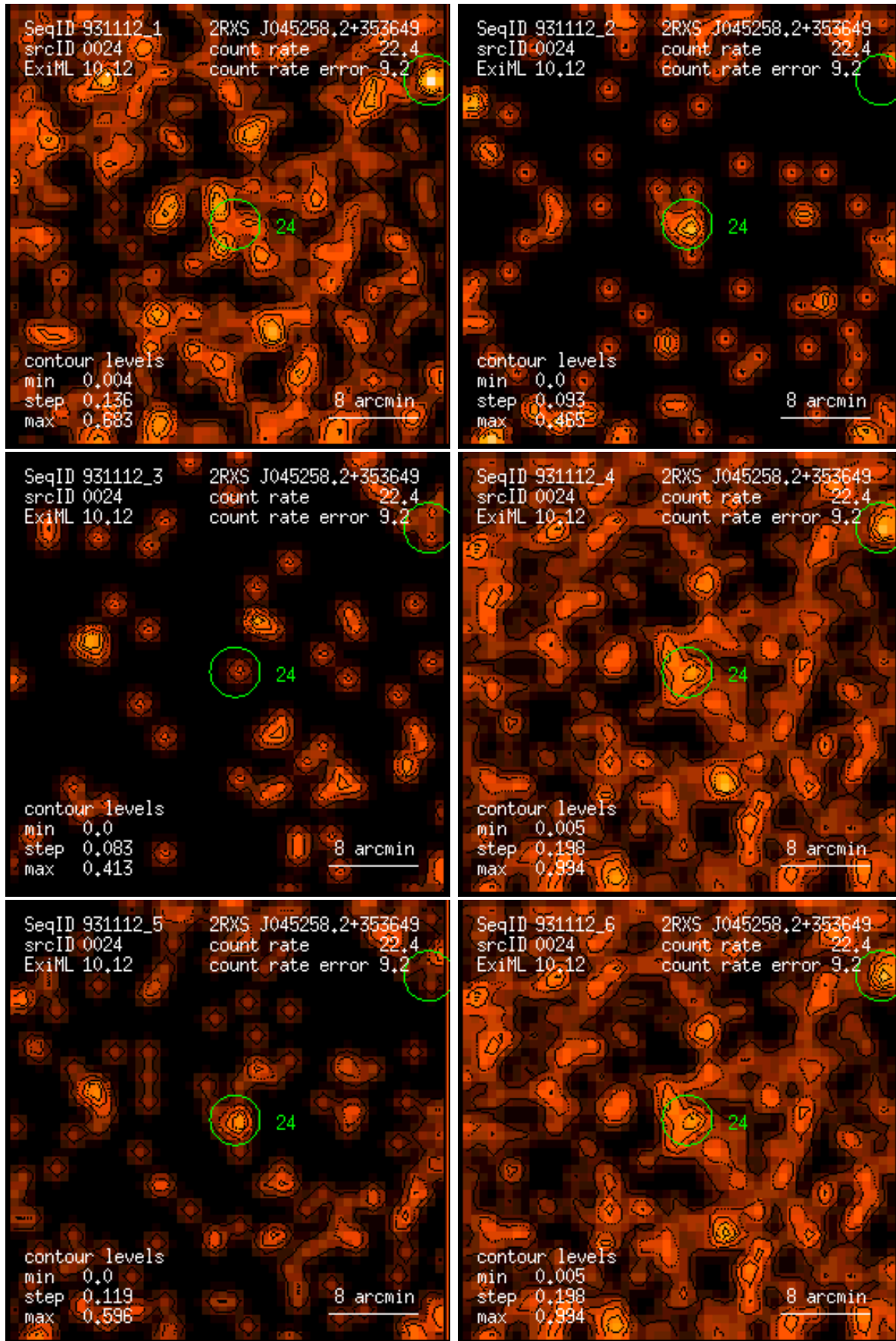
Figure 24: RASS 931112: detection 0024: band rate images, Gaussian filter: (1) PSPC channels 11 – 41, (2) 52 – 90, (3) 91 – 201, (4) 11 – 235, (5) 52 – 201, (6) 11 – 201. Broad band rates in counts/ks. Band rate contour levels in counts/ks/arcmin 2 .
