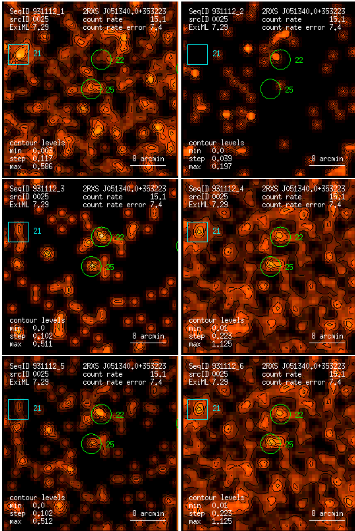
Figure 25: RASS 931112: detection 0025: band rate images, Gaussian filter: (1) PSPC channels 11 – 41, (2) 52 – 90, (3) 91 – 201, (4) 11 – 235, (5) 52 – 201, (6) 11 – 201. Broad band rates in counts/ks. Band rate contour levels in counts/ks/arcmin 2 .
