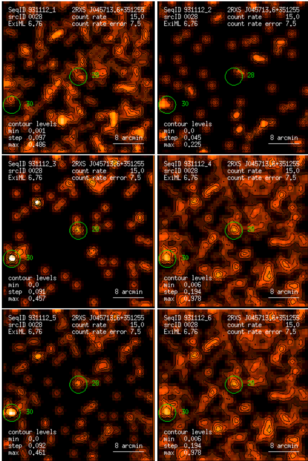
Figure 28: RASS 931112: detection 0028: band rate images, Gaussian filter: (1) PSPC channels 11 – 41, (2) 52 – 90, (3) 91 – 201, (4) 11 – 235, (5) 52 – 201, (6) 11 – 201. Broad band rates in counts/ks. Band rate contour levels in counts/ks/arcmin 2 .
