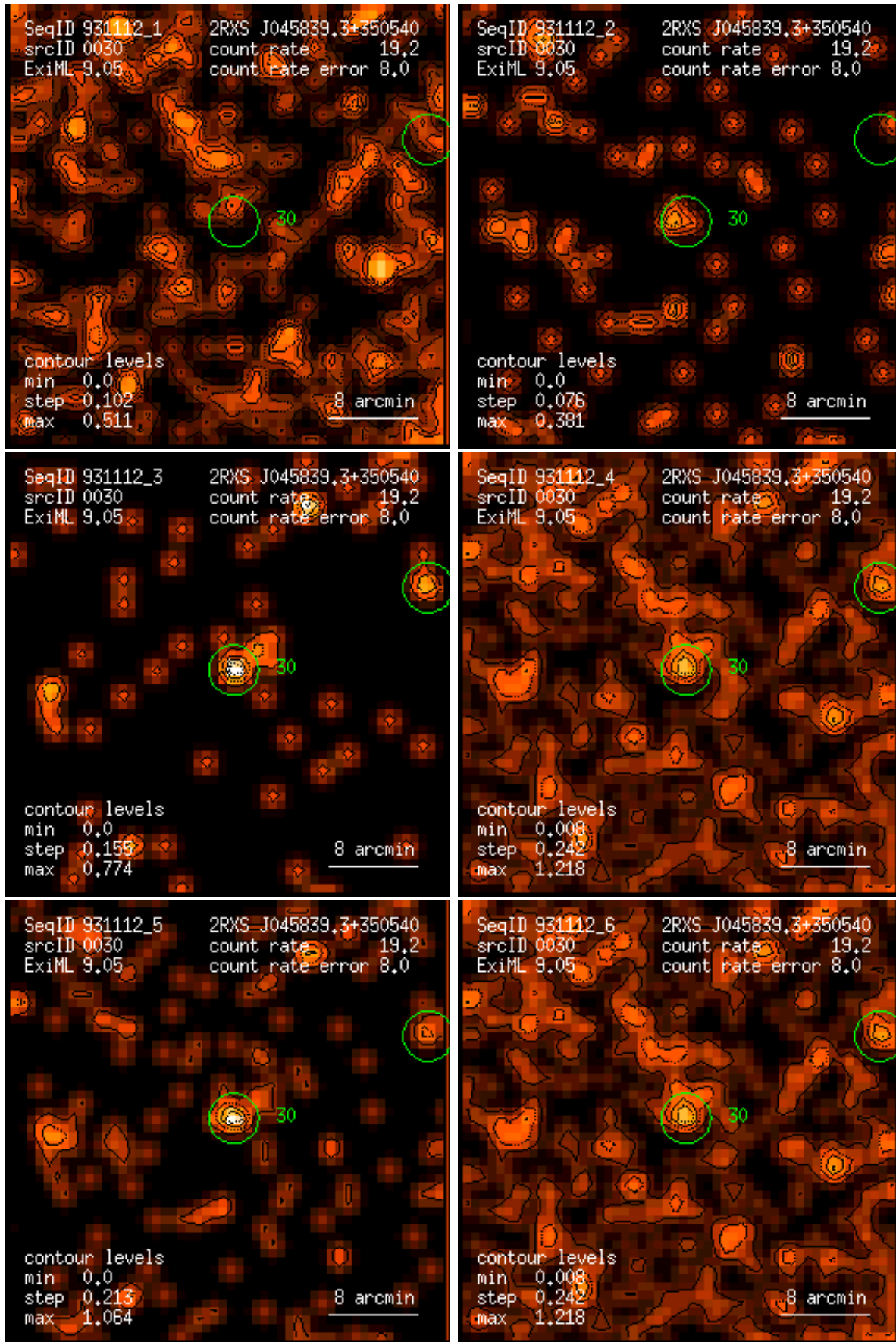
Figure 30: RASS 931112: detection 0030: band rate images, Gaussian filter: (1) PSPC channels 11 – 41, (2) 52 – 90, (3) 91 – 201, (4) 11 – 235, (5) 52 – 201, (6) 11 – 201. Broad band rates in counts/ks. Band rate contour levels in counts/ks/arcmin 2 .
