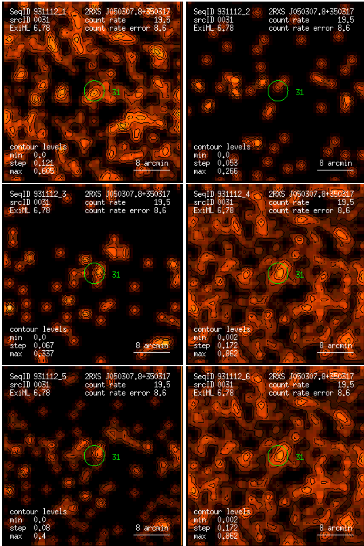
Figure 31: RASS 931112: detection 0031: band rate images, Gaussian filter: (1) PSPC channels 11 – 41, (2) 52 – 90, (3) 91 – 201, (4) 11 – 235, (5) 52 – 201, (6) 11 – 201. Broad band rates in counts/ks. Band rate contour levels in counts/ks/arcmin 2 .
