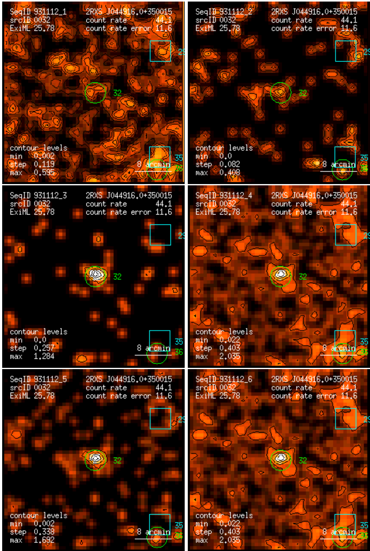
Figure 32: RASS 931112: detection 0032: band rate images, Gaussian filter: (1) PSPC channels 11 – 41, (2) 52 – 90, (3) 91 – 201, (4) 11 – 235, (5) 52 – 201, (6) 11 – 201. Broad band rates in counts/ks. Band rate contour levels in counts/ks/arcmin 2 .
