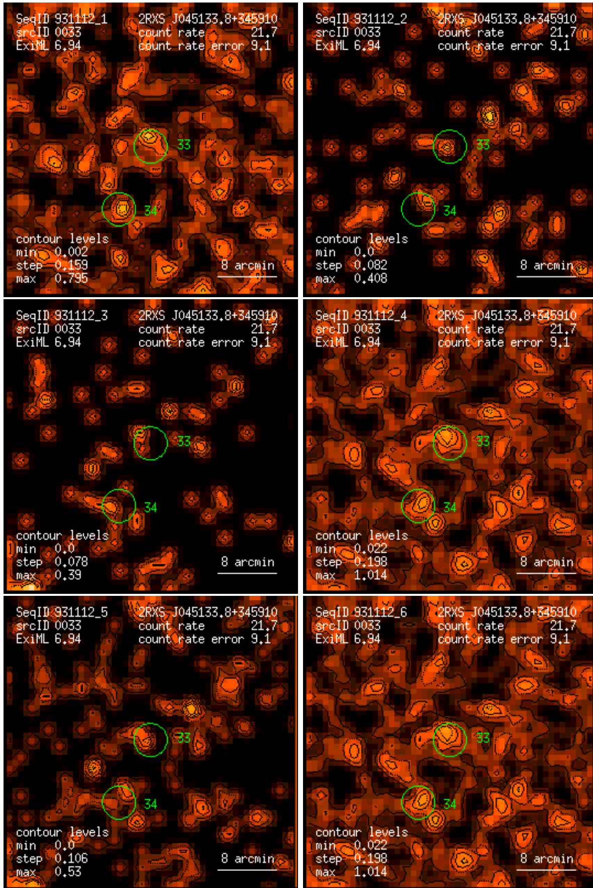
Figure 33: RASS 931112: detection 0033: band rate images, Gaussian filter: (1) PSPC channels 11 – 41, (2) 52 – 90, (3) 91 – 201, (4) 11 – 235, (5) 52 – 201, (6) 11 – 201. Broad band rates in counts/ks. Band rate contour levels in counts/ks/arcmin 2 .
