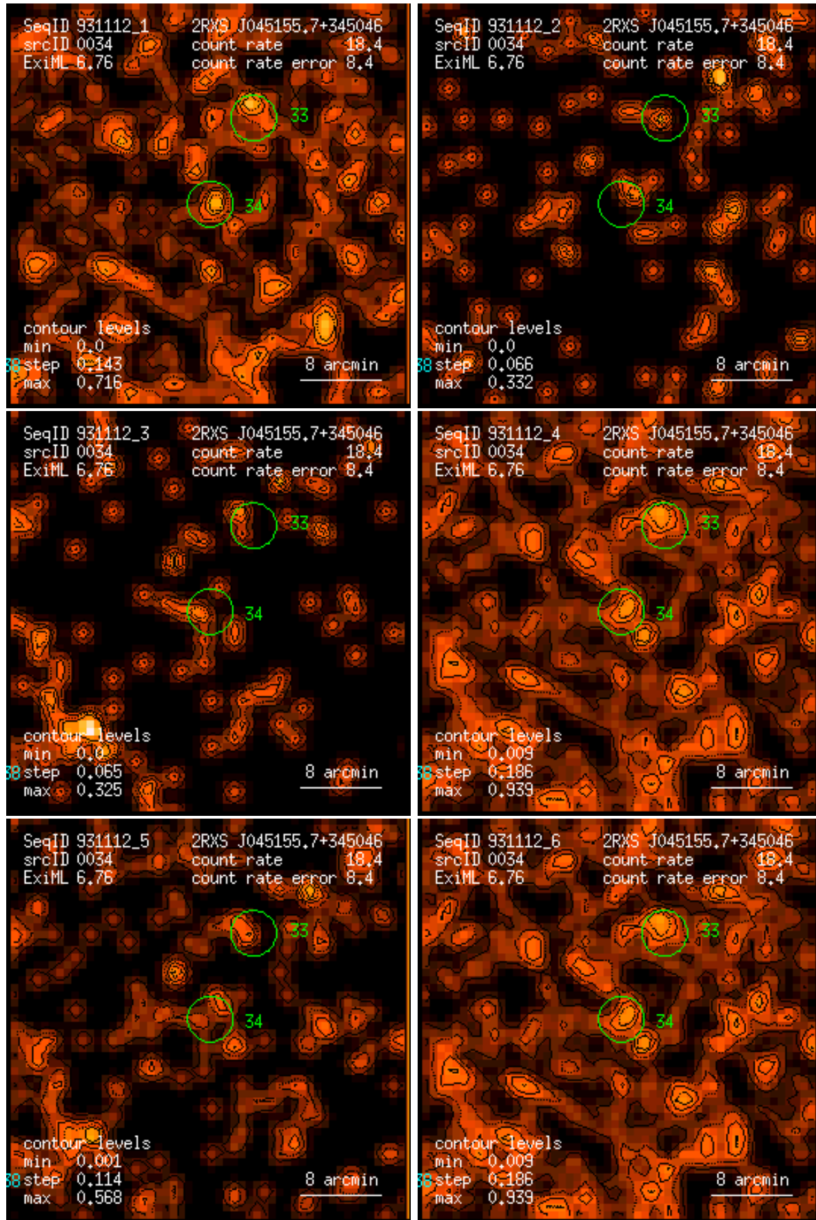
Figure 34: RASS 931112: detection 0034: band rate images, Gaussian filter: (1) PSPC channels 11 – 41, (2) 52 – 90, (3) 91 – 201, (4) 11 – 235, (5) 52 – 201, (6) 11 – 201. Broad band rates in counts/ks. Band rate contour levels in counts/ks/arcmin 2 .
