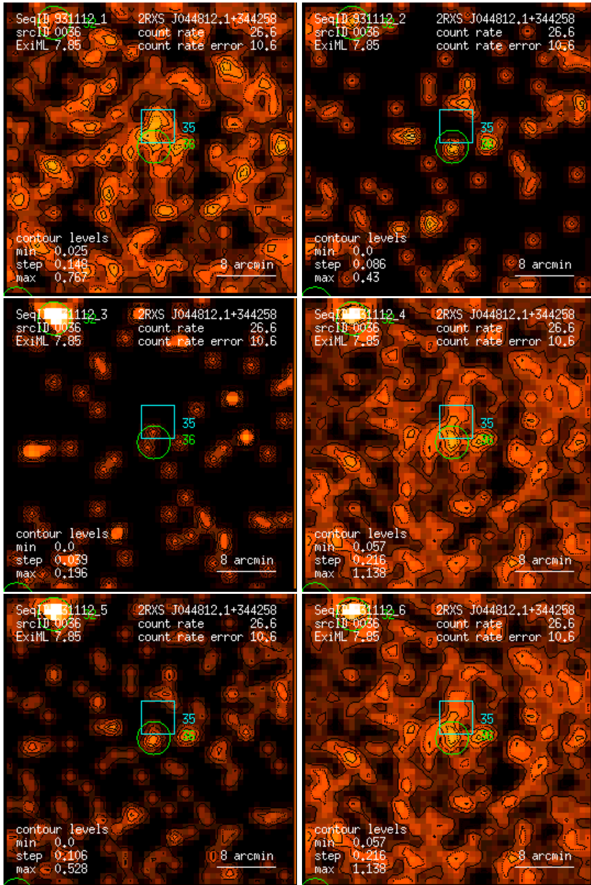
Figure 36: RASS 931112: detection 0036: band rate images, Gaussian filter: (1) PSPC channels 11 – 41, (2) 52 – 90, (3) 91 – 201, (4) 11 – 235, (5) 52 – 201, (6) 11 – 201. Broad band rates in counts/ks. Band rate contour levels in counts/ks/arcmin 2 .
