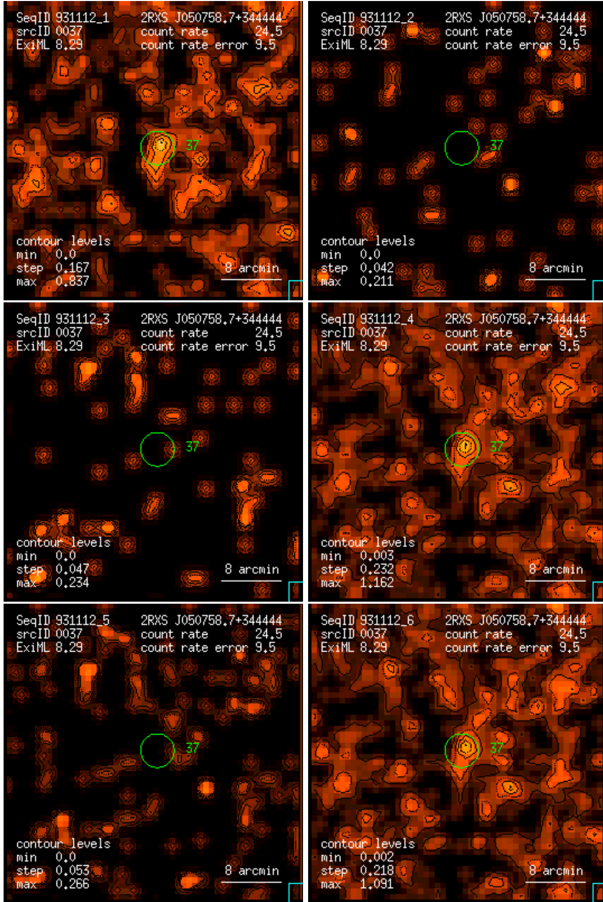
Figure 37: RASS 931112: detection 0037: band rate images, Gaussian filter: (1) PSPC channels 11 – 41, (2) 52 – 90, (3) 91 – 201, (4) 11 – 235, (5) 52 – 201, (6) 11 – 201. Broad band rates in counts/ks. Band rate contour levels in counts/ks/arcmin 2 .
