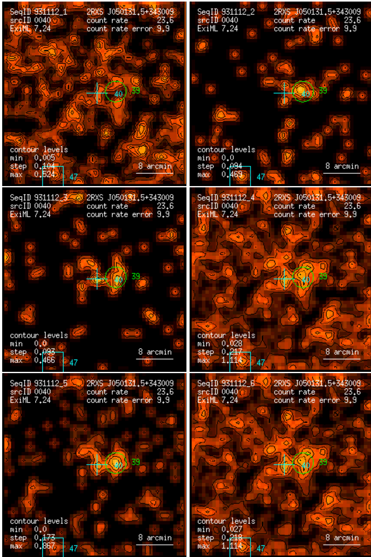
Figure 40: RASS 931112: detection 0040: band rate images, Gaussian filter: (1) PSPC channels 11 – 41, (2) 52 – 90, (3) 91 – 201, (4) 11 – 235, (5) 52 – 201, (6) 11 – 201. Broad band rates in counts/ks. Band rate contour levels in counts/ks/arcmin 2 .
