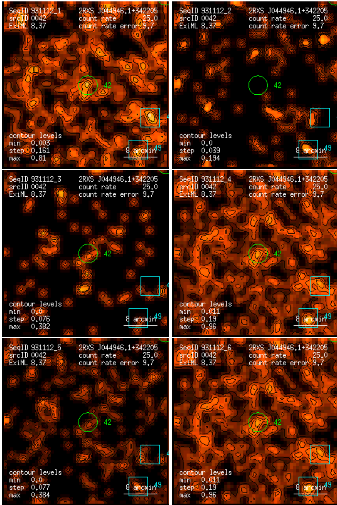
Figure 42: RASS 931112: detection 0042: band rate images, Gaussian filter: (1) PSPC channels 11 – 41, (2) 52 – 90, (3) 91 – 201, (4) 11 – 235, (5) 52 – 201, (6) 11 – 201. Broad band rates in counts/ks. Band rate contour levels in counts/ks/arcmin 2 .
